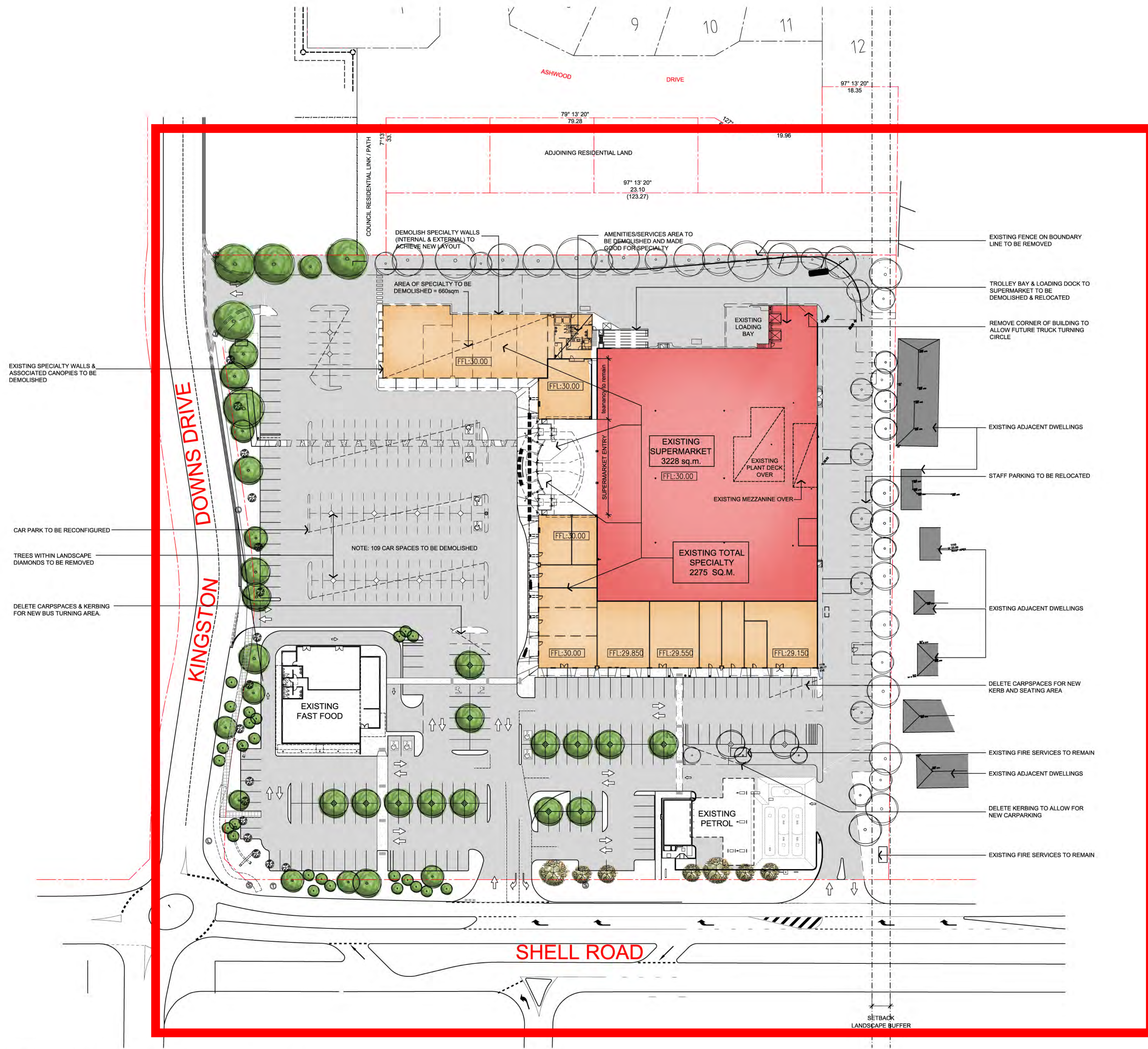
EXISTING SITE & DEMOLITION PLAN SCALE: 1:500
